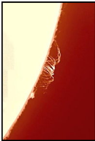
Solar Magnetic Loops November 2021
