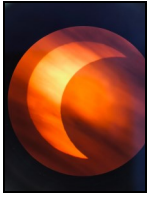
Partial Eclipse June 2021
